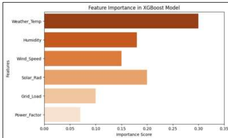
Figure 11. A feature importance plot for XGBoost model
